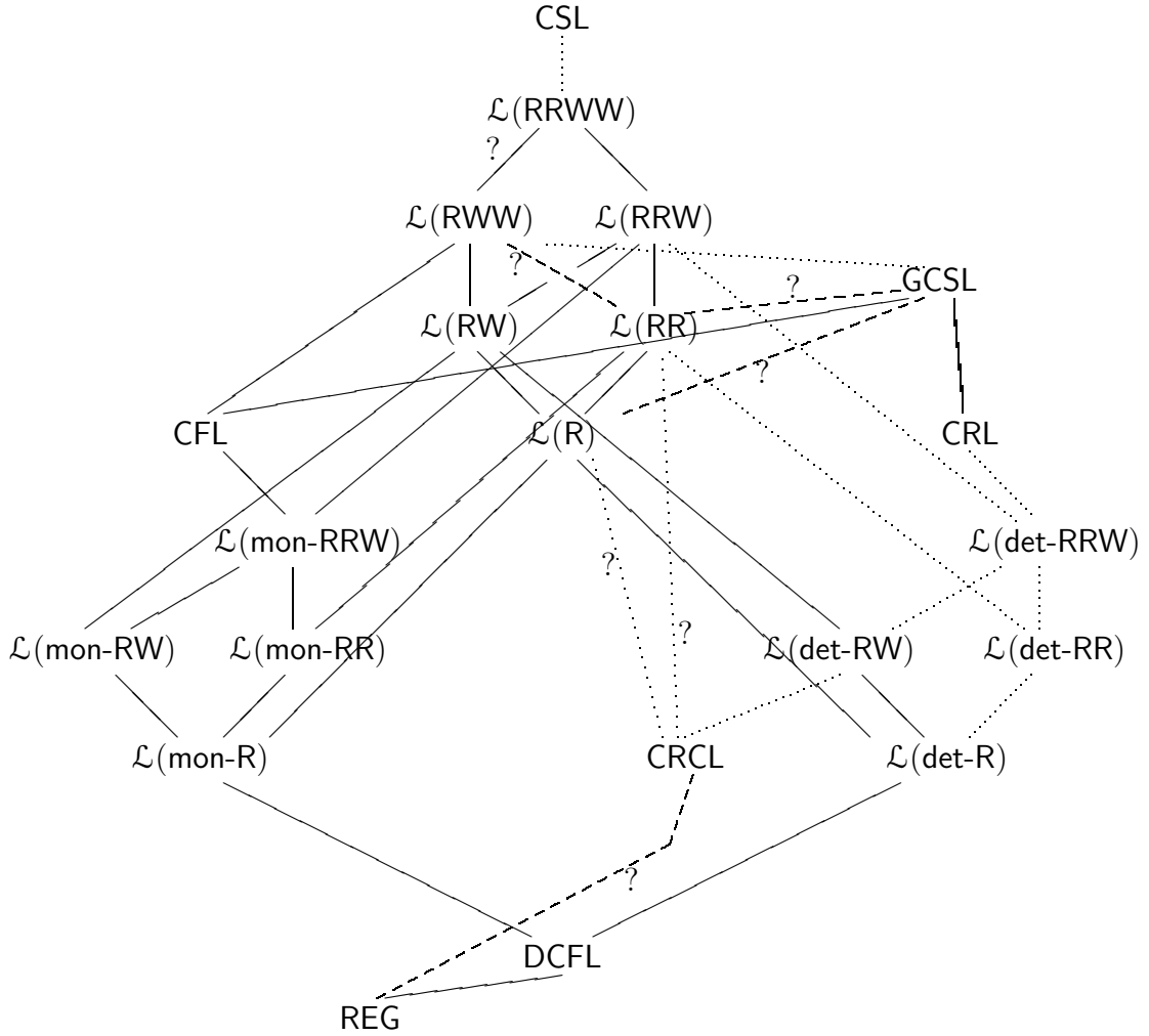
Figure 5.1: Relations among the language classes considered as of Section 5.1
