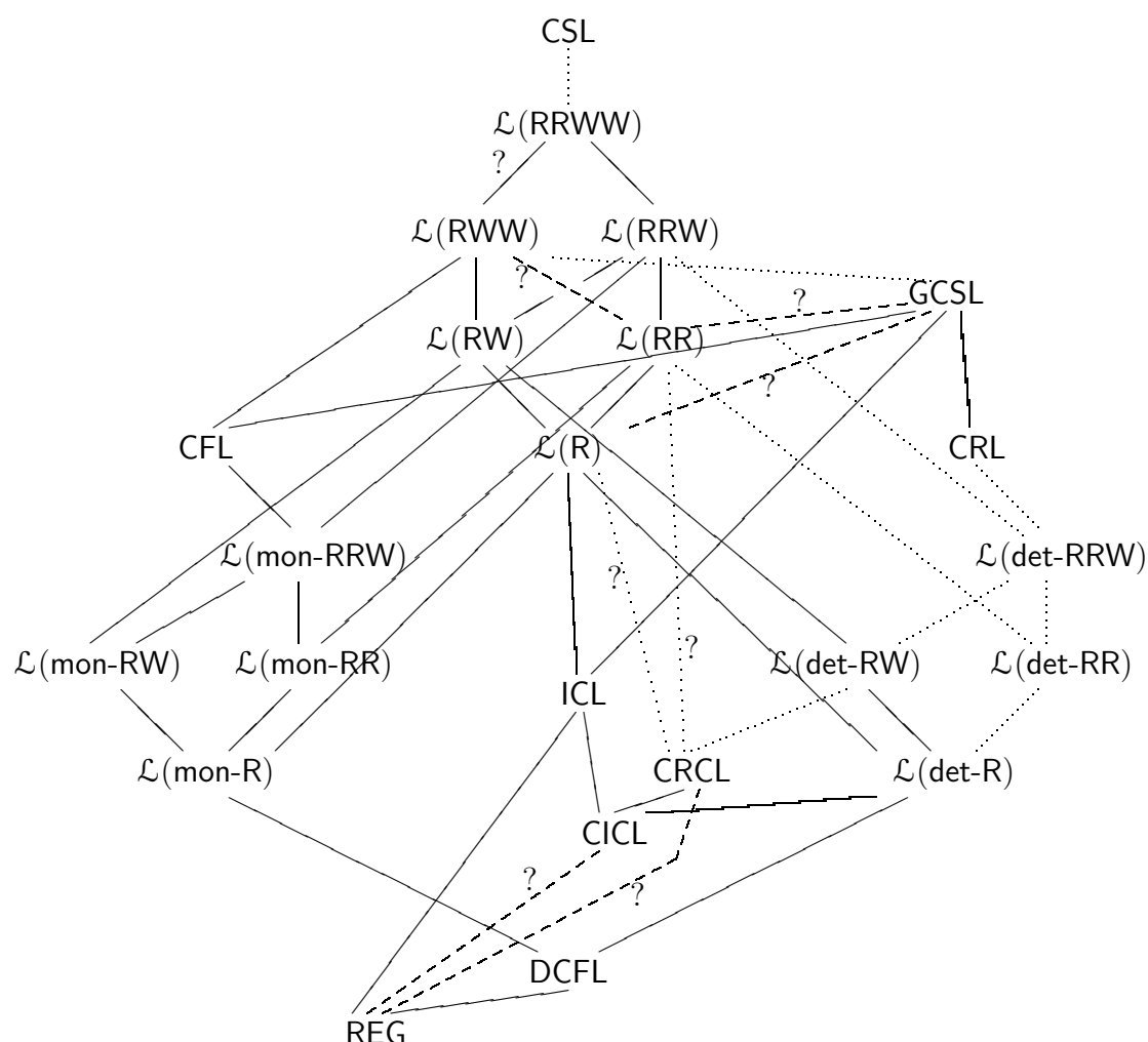
Figure 6.1: Relations among the language classes considered as of Section 6.1
