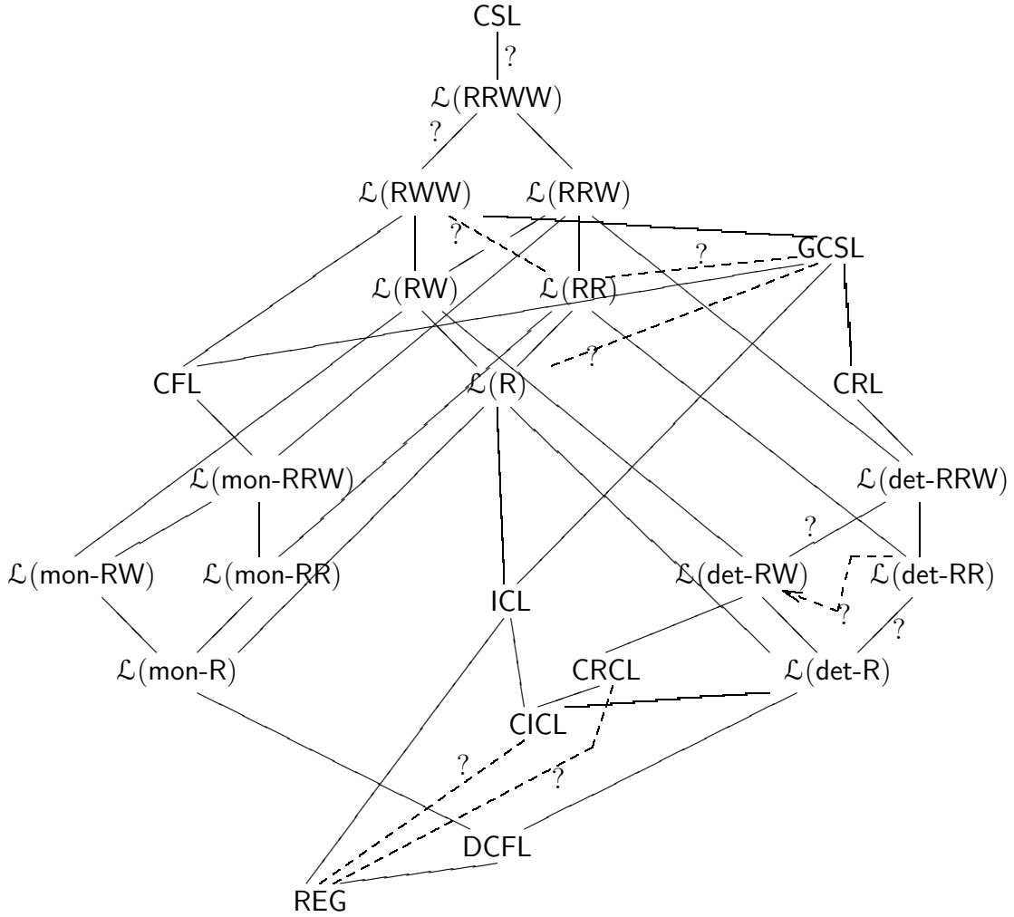
Figure 7.2: Summary of the relations among the language classes considered
